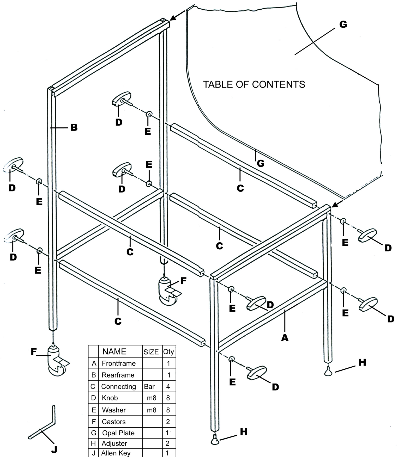
CAMBO MINI-ST SHOOTING TABLE MOUNTING INSTRUCTION
